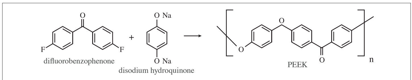
Figure 1: PEEK synthesis and immediate precursors. PEEK is synthesized most immediately from difluorobenzophenone and disodium hydroquinone. Note that PEEK does not contain fluorine and therefore is not a fluoropolymer. PEEK is a halogen-free material. [1]
